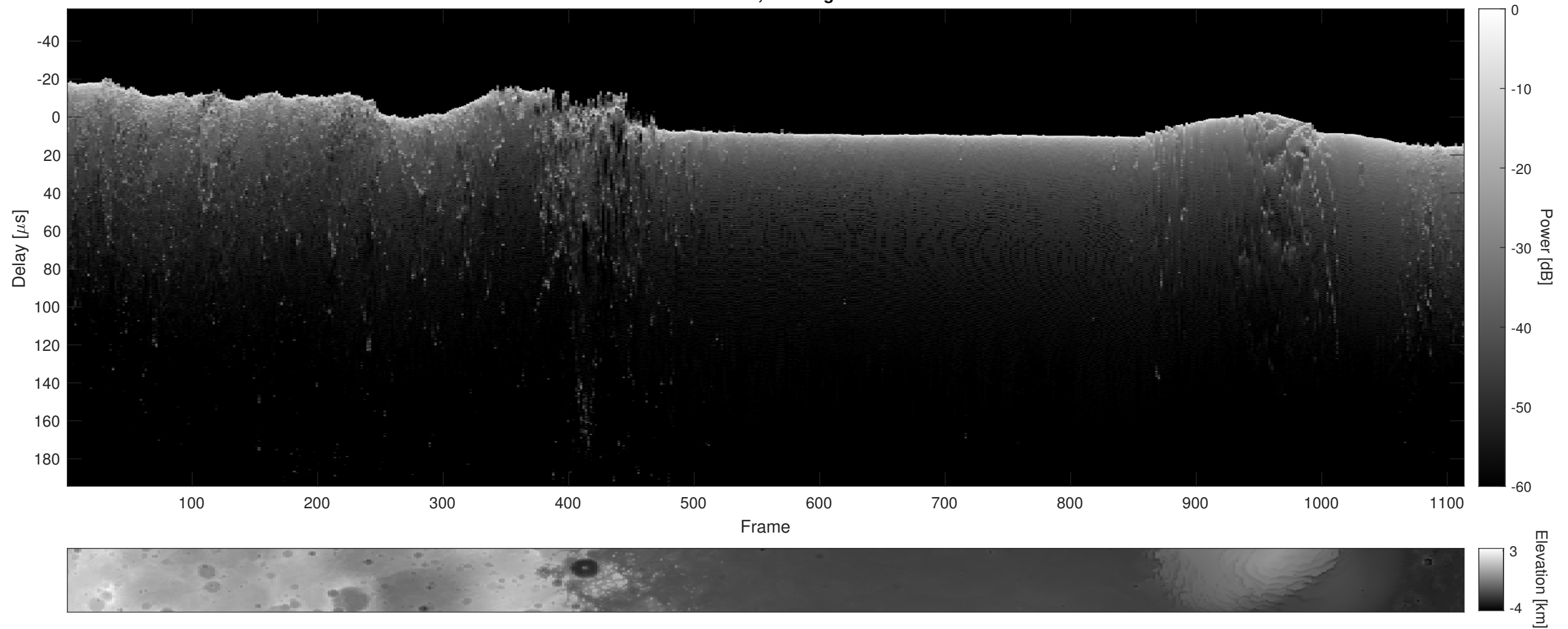
Orbit 14180, Cluttergram
