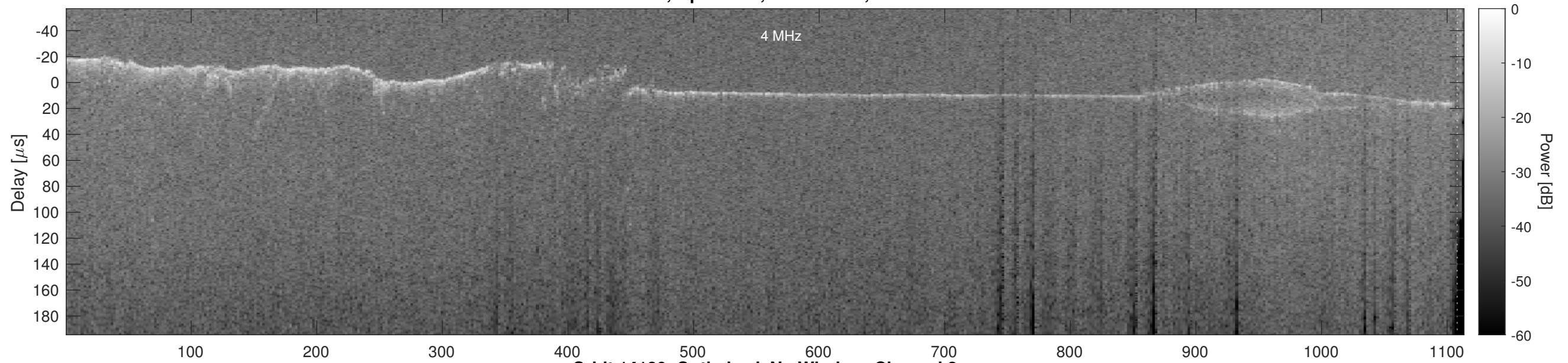
Orbit 14180, Optimized, No Window, Channel 2
