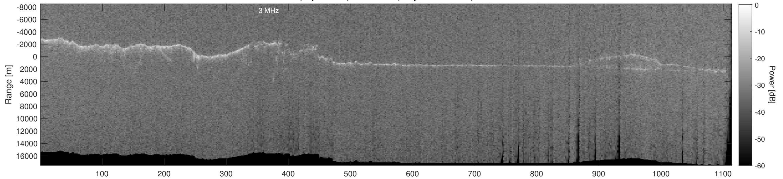
Orbit 14180, Depth-Corrected Cluttergram
