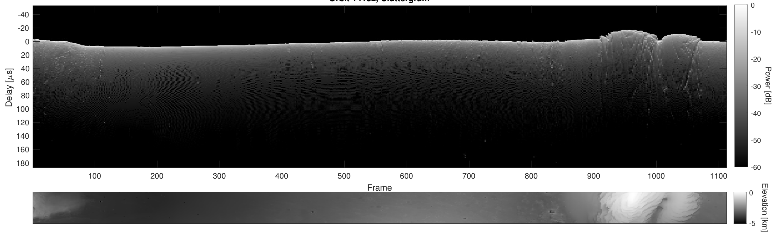
Orbit 14182, Cluttergram
