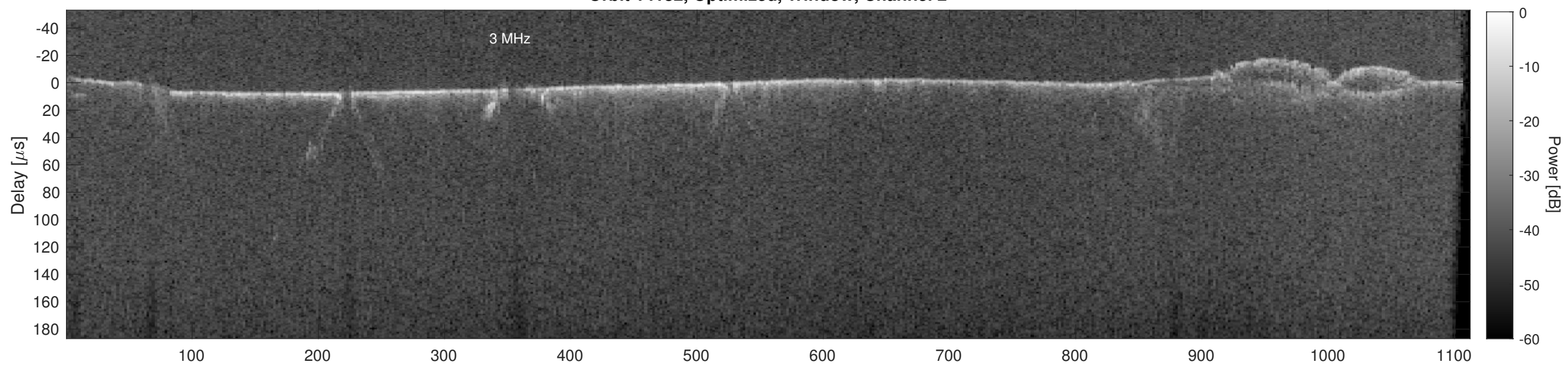
Orbit 14182, Cluttergram
