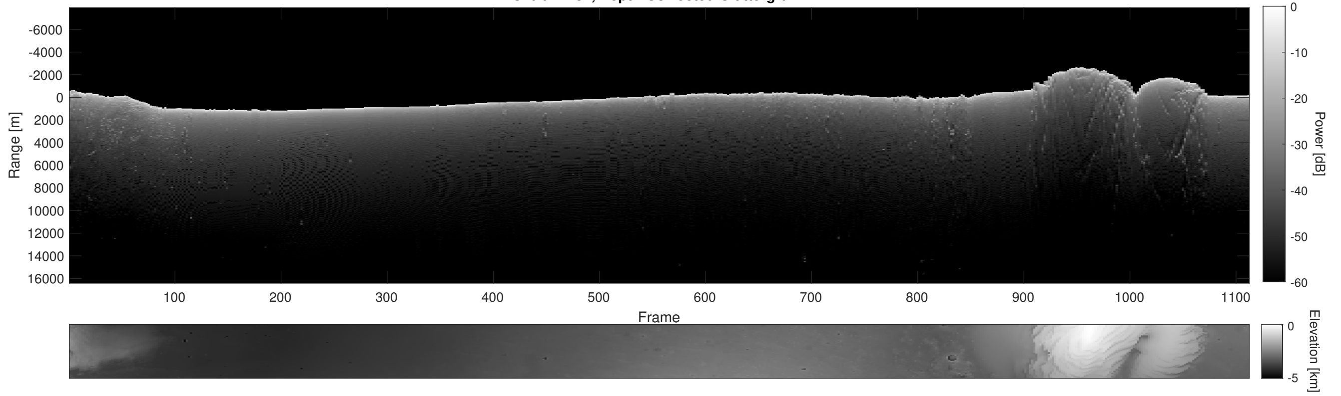
Orbit 14182, Depth-Corrected Cluttergram
