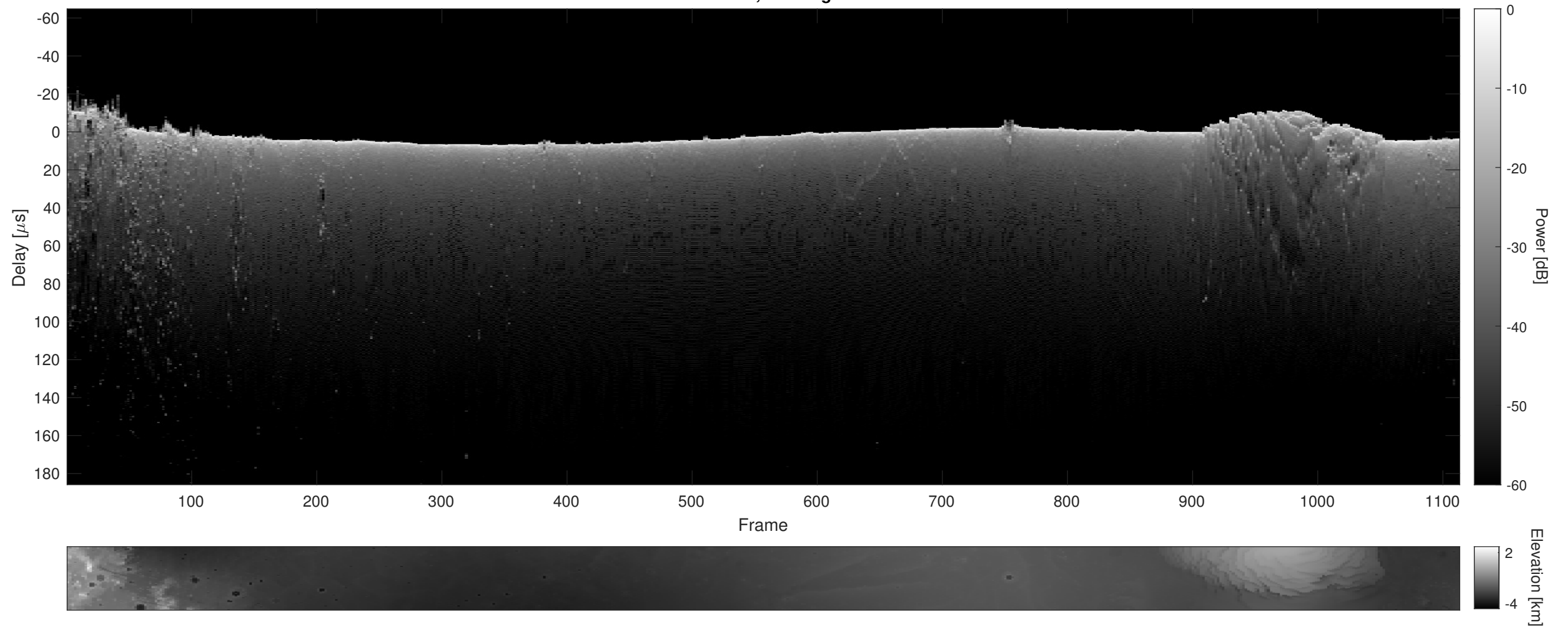
Orbit 14183, Cluttergram
