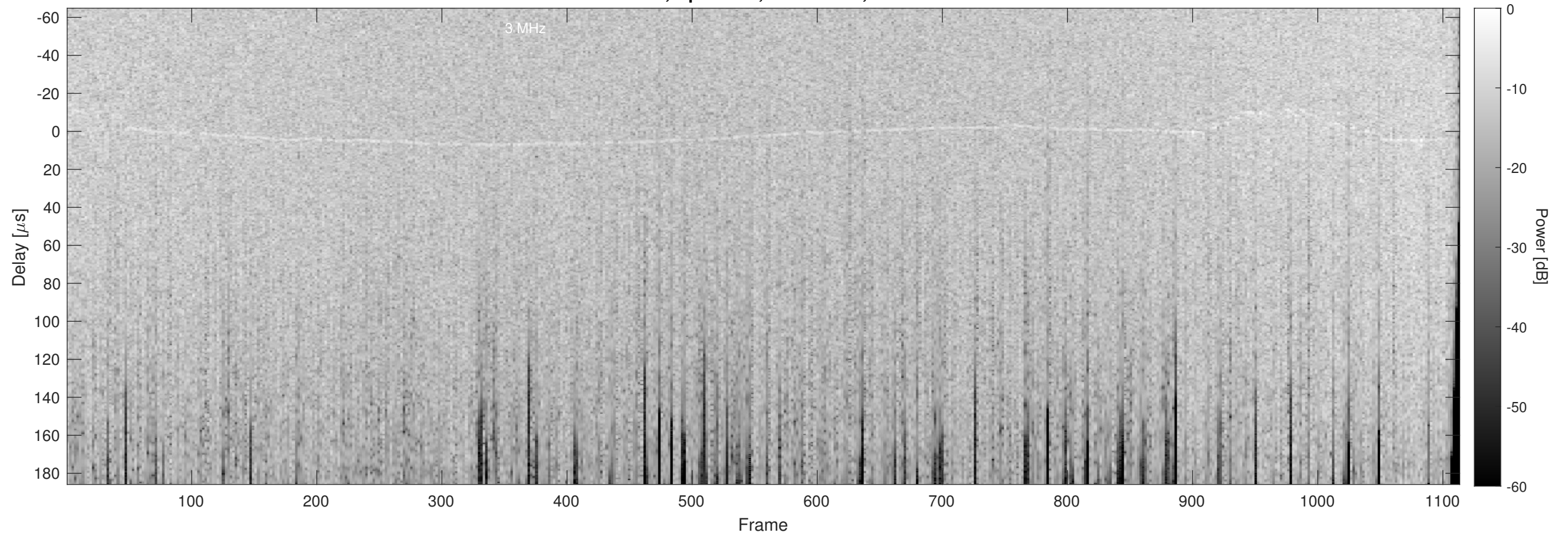
Orbit 14183, Optimized, No Window, Channel 2
