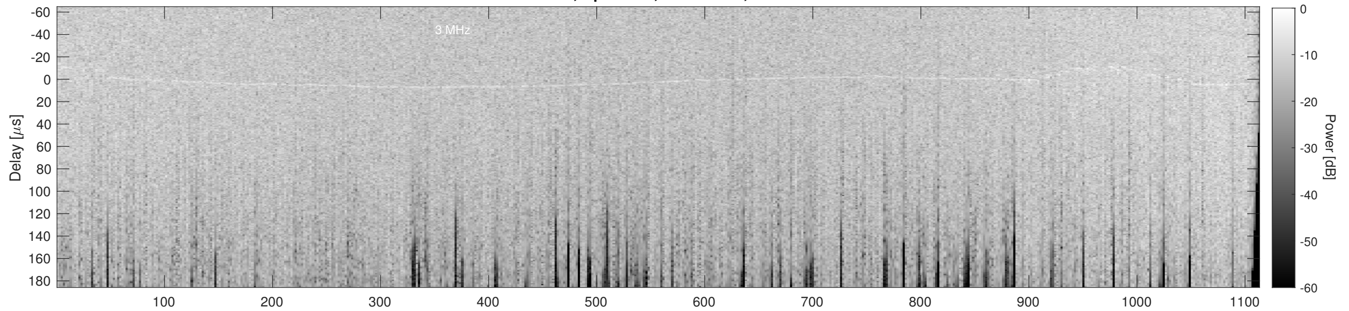
Orbit 14183, Cluttergram
