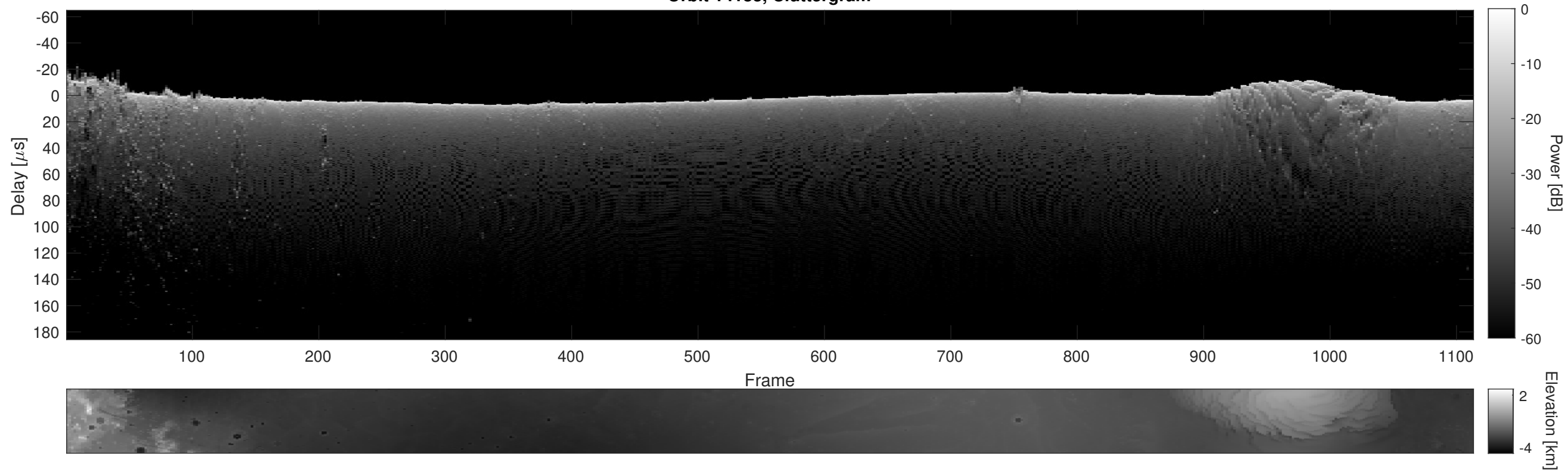
Orbit 14183, Cluttergram
