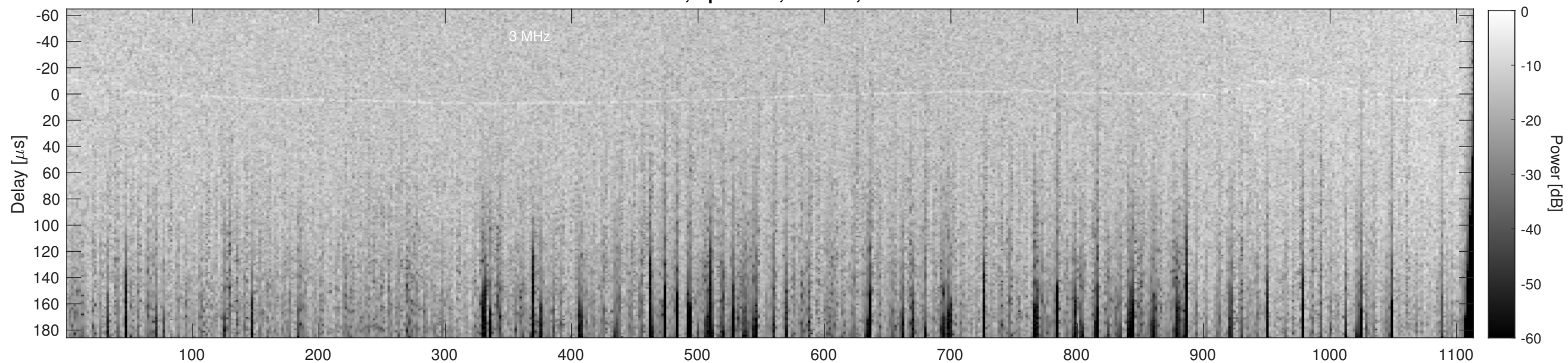
Orbit 14183, Cluttergram
