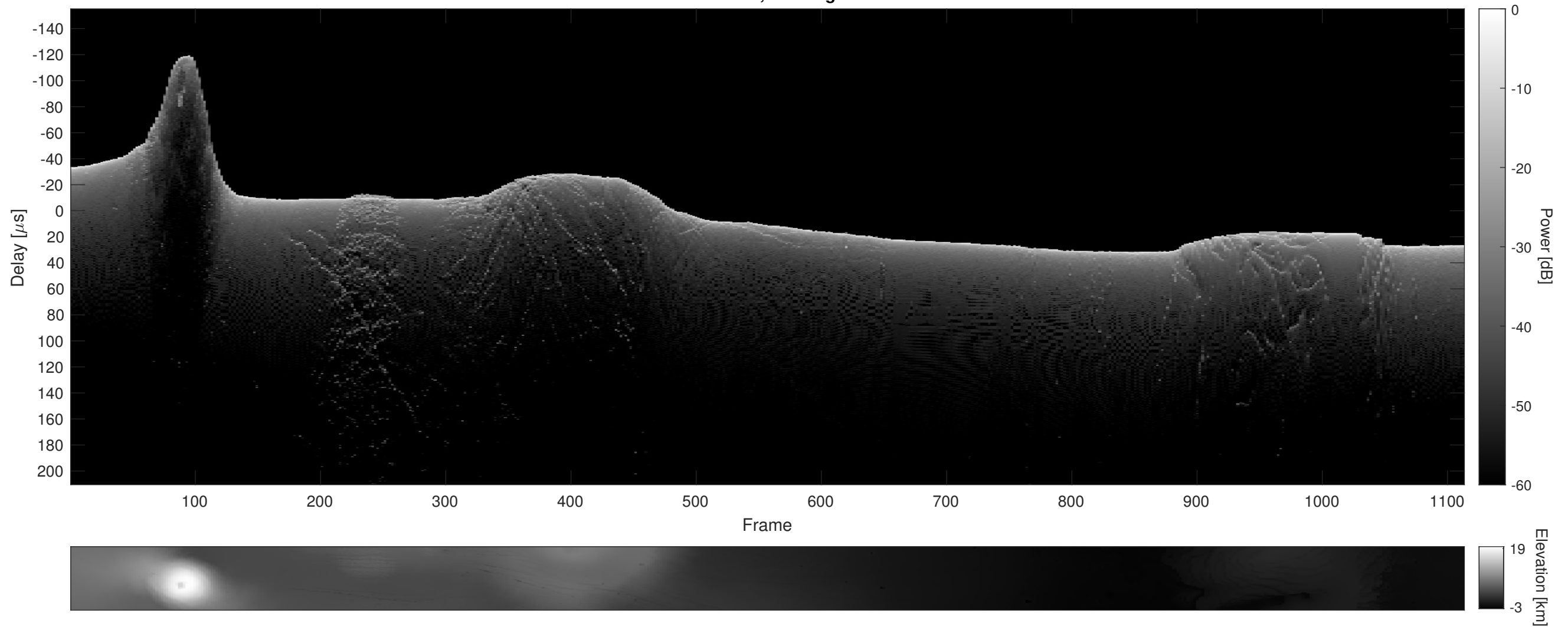
Orbit 14185, Cluttergram
