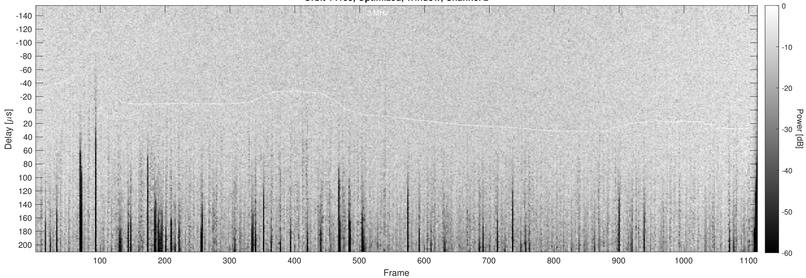
Orbit 14185, Optimized, Window, Channel 2
