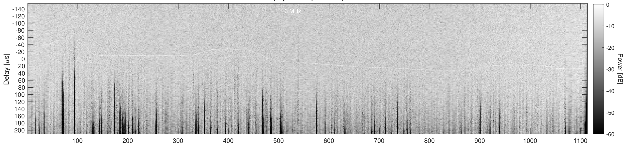
Orbit 14185, Cluttergram
