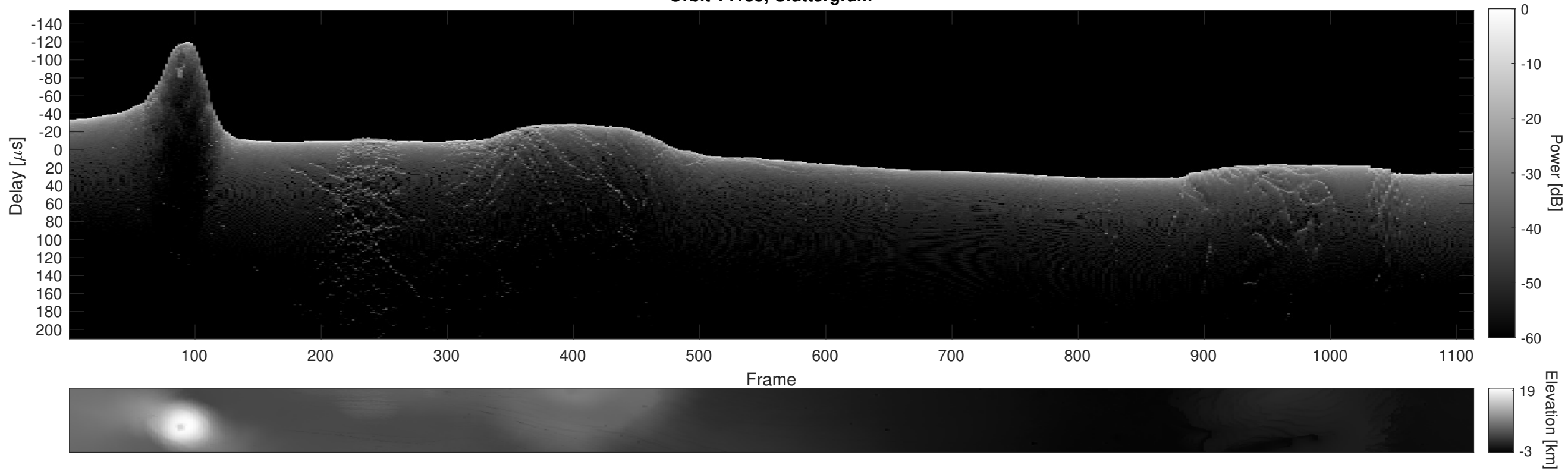
Orbit 14185, Cluttergram
