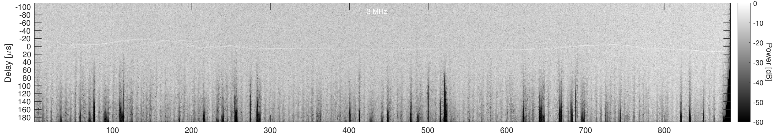
Orbit 14187, Cluttergram
