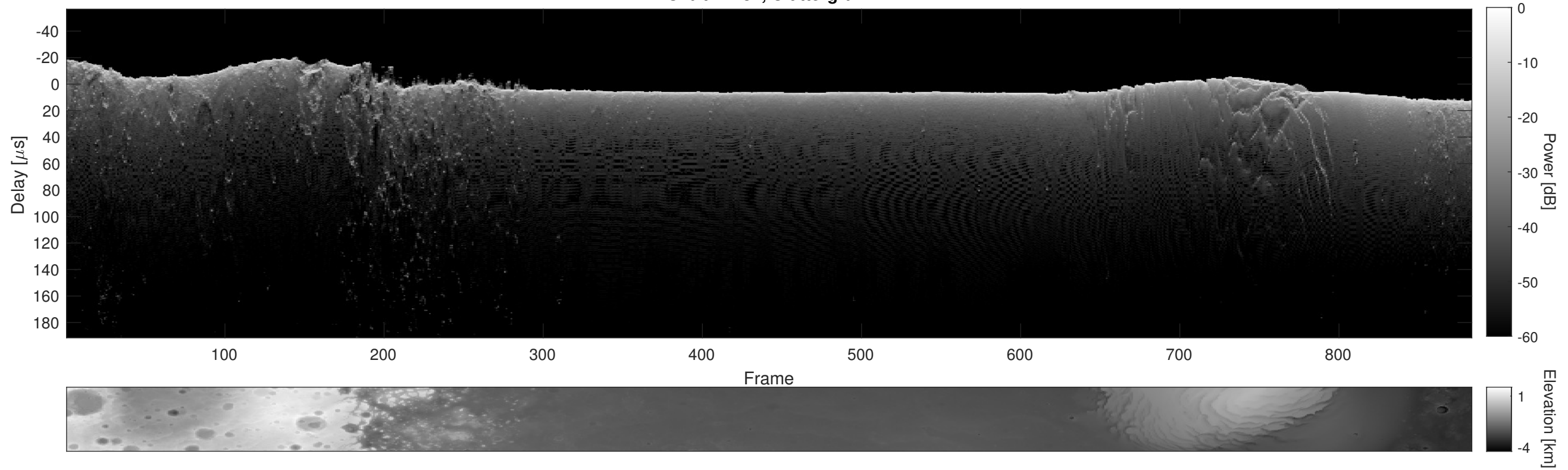
Orbit 14187, Cluttergram
