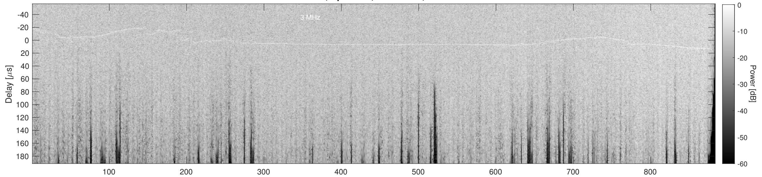
Orbit 14187, Cluttergram
