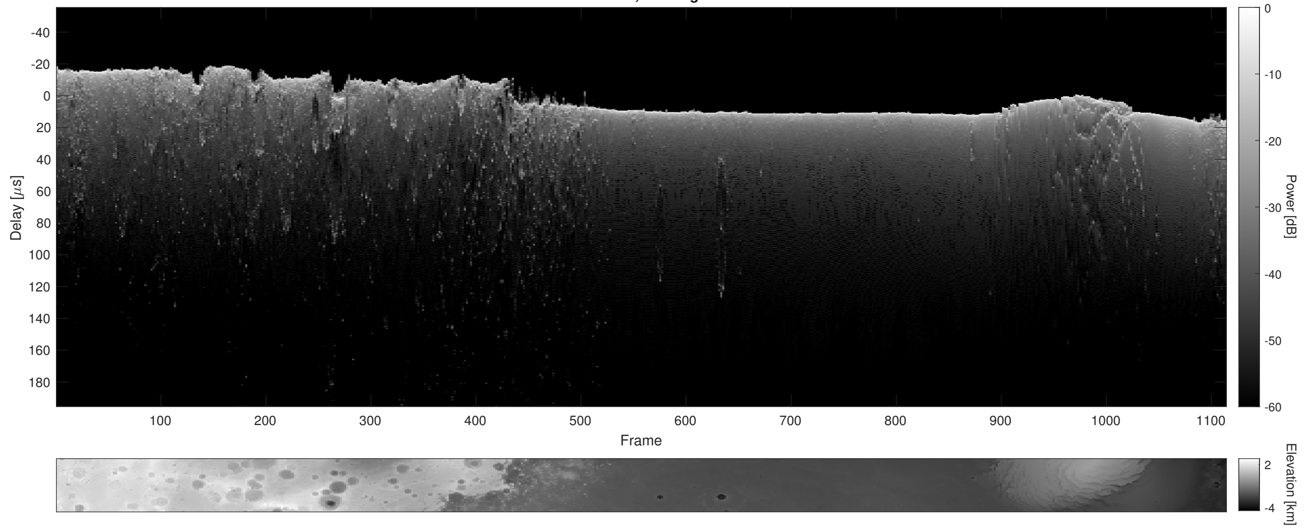
Orbit 14194, Cluttergram
