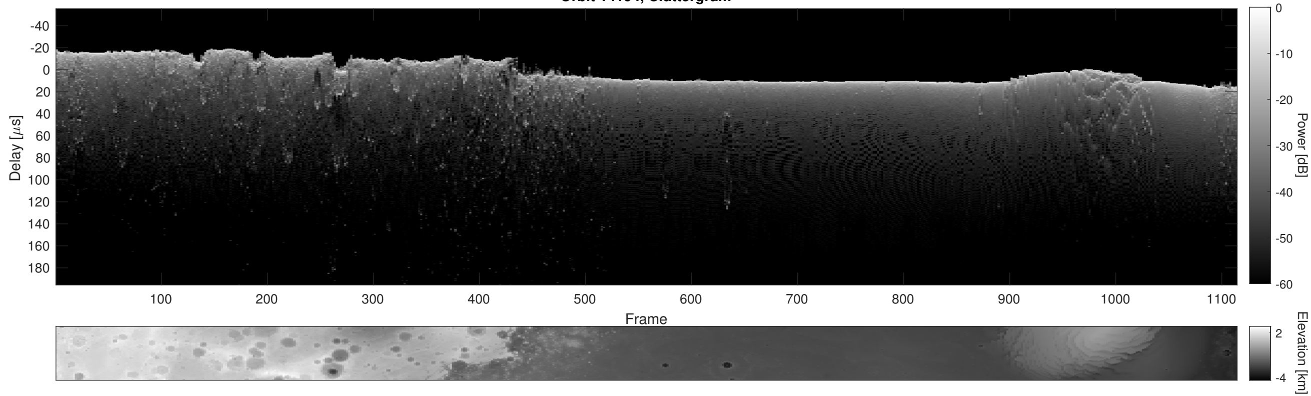
Orbit 14194, Cluttergram
