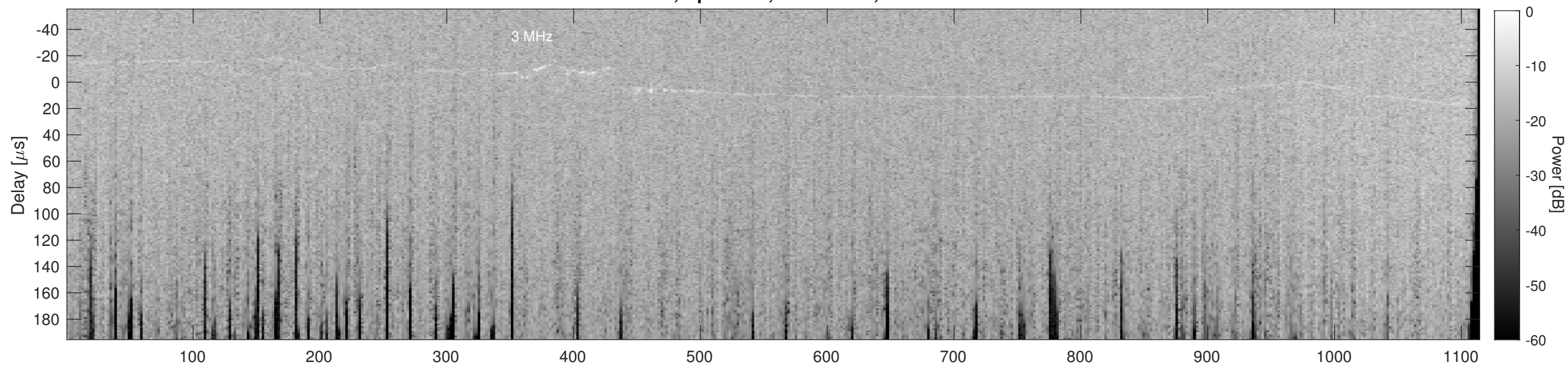
Orbit 14194, Cluttergram
