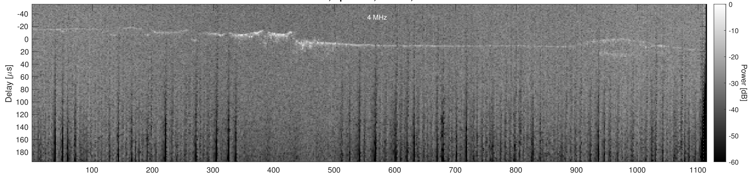
Orbit 14194, Optimized, Window, Channel 2
