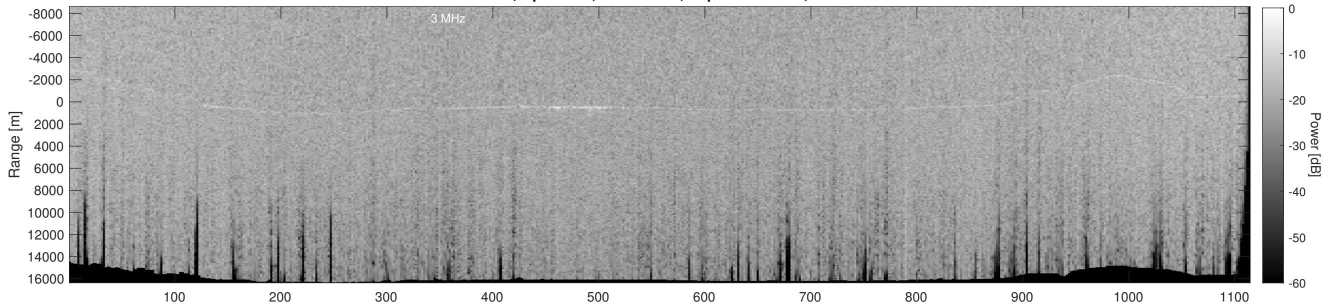
Orbit 14195, Depth-Corrected Cluttergram
