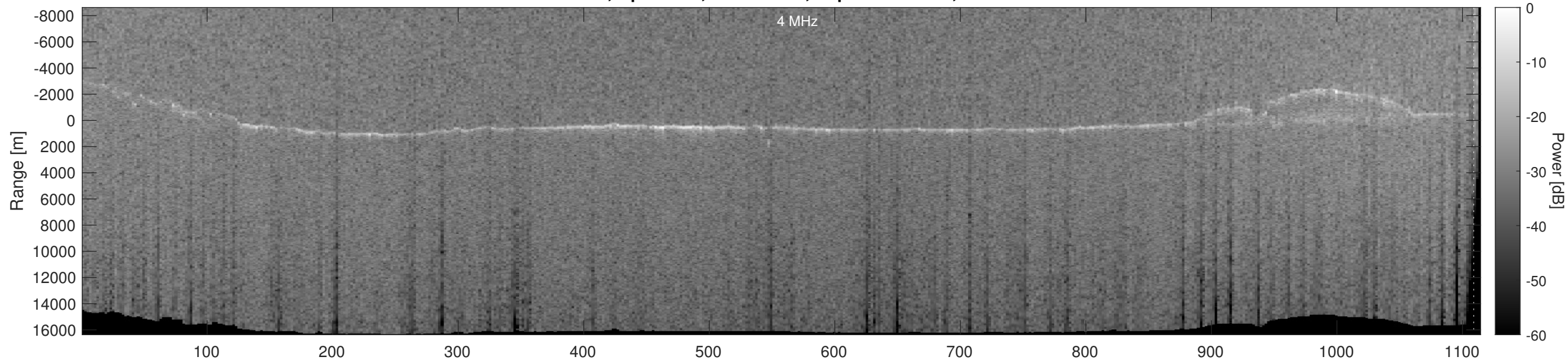
Orbit 14195, Optimized, No Window, Depth-Corrected, Channel 2
