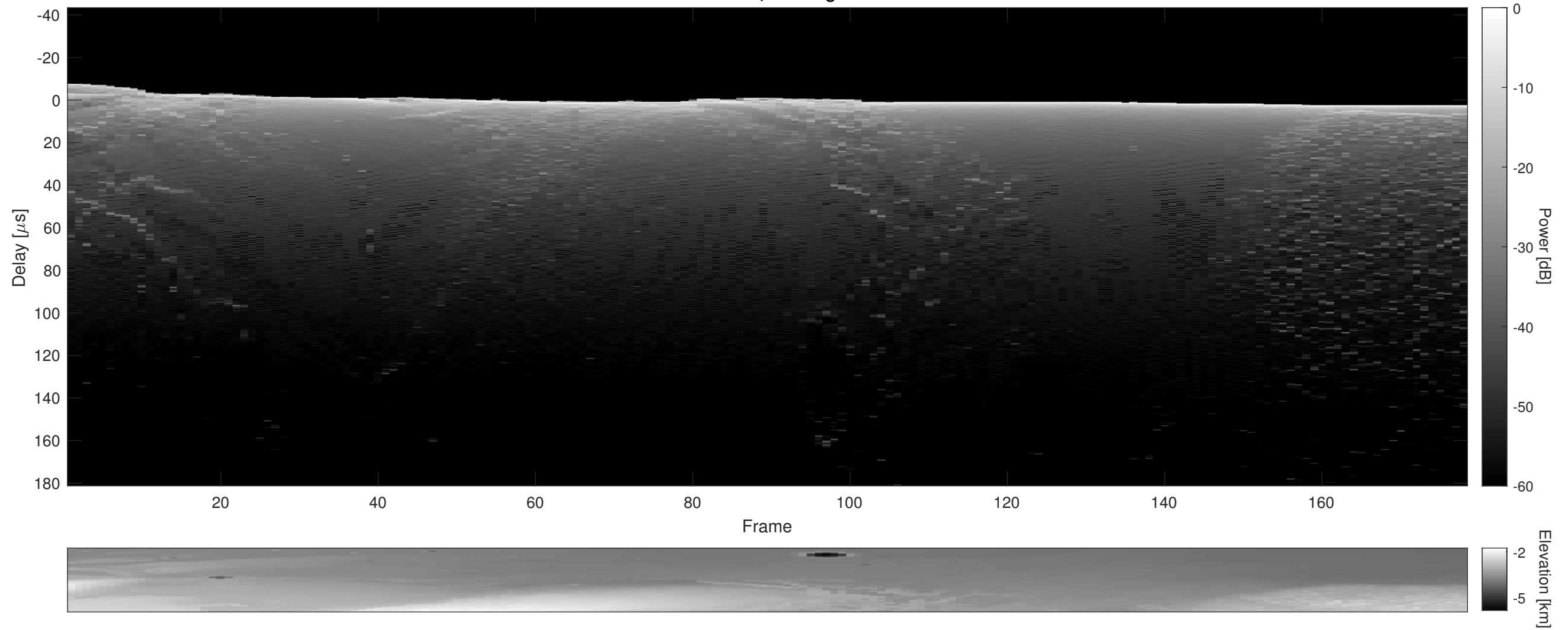
Orbit 14196, Cluttergram
