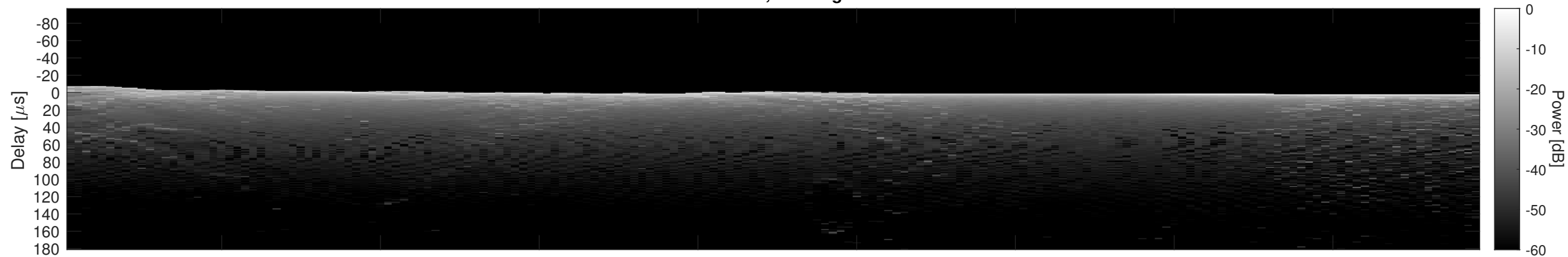
Orbit 14196, Cluttergram
