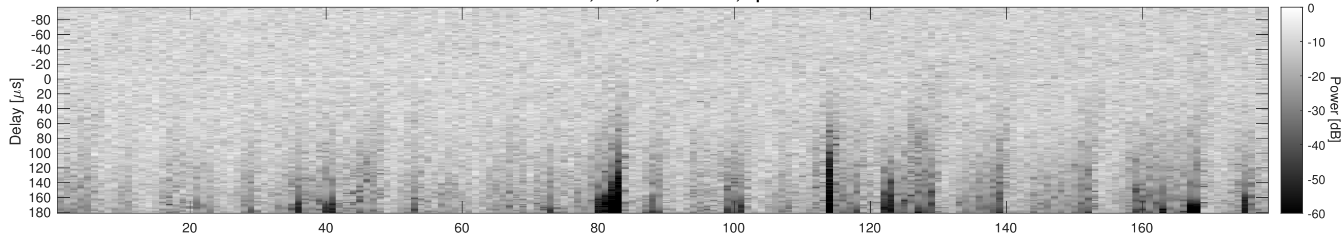
Orbit 14196, Cluttergram
