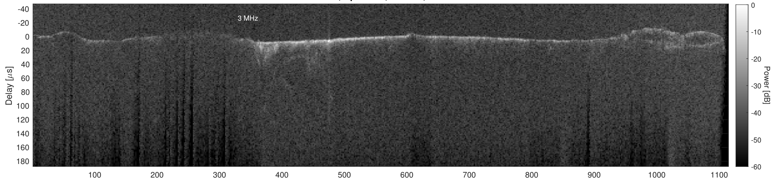
Orbit 14203, Cluttergram
