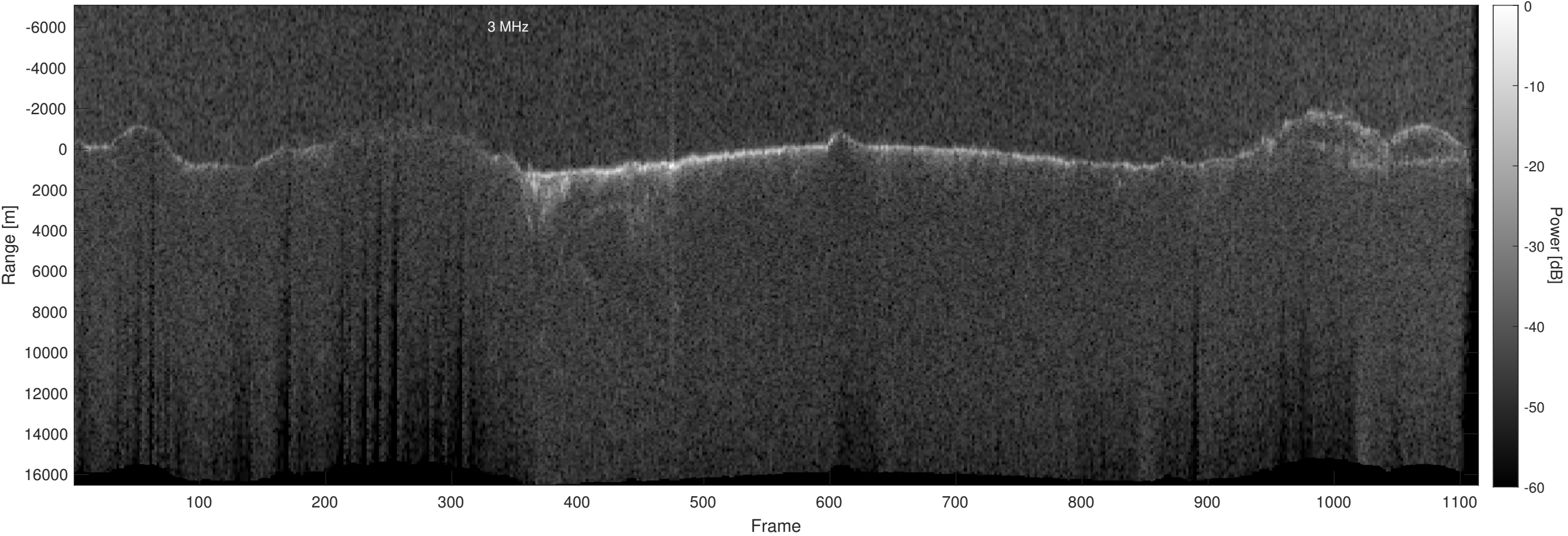
Orbit 14203, Optimized, Window, Depth-Corrected, Channel 2
