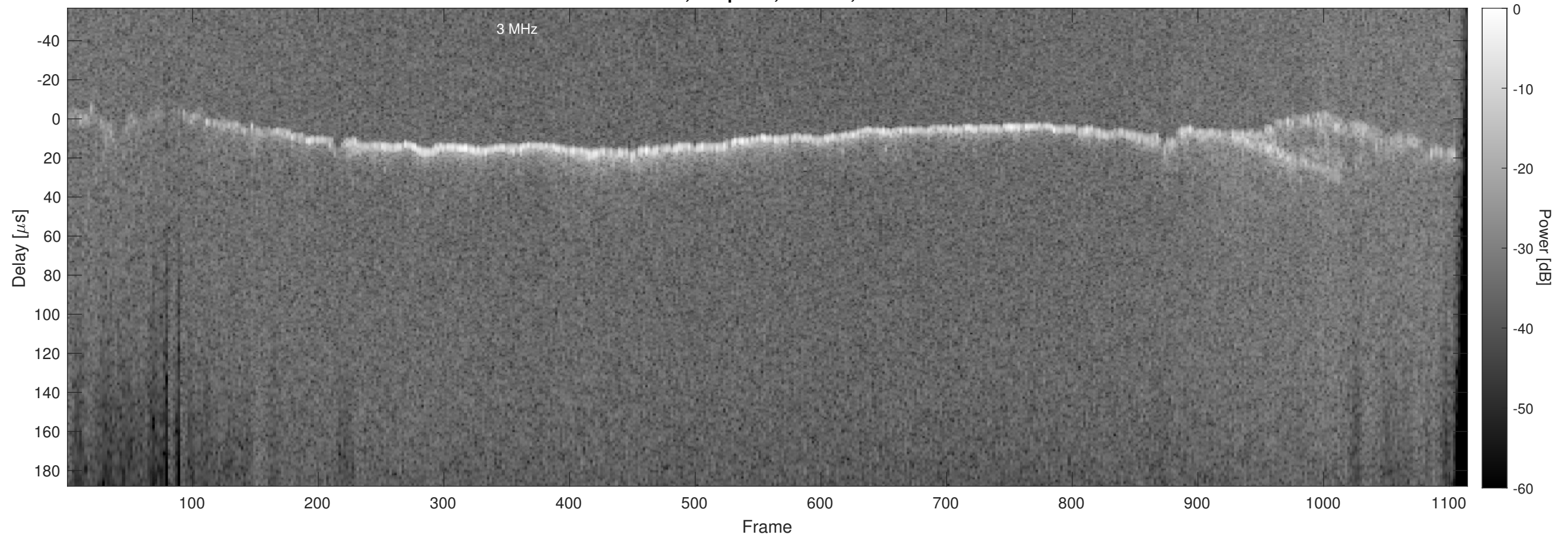
Orbit 14204, Chapman, Window, Channel 2
