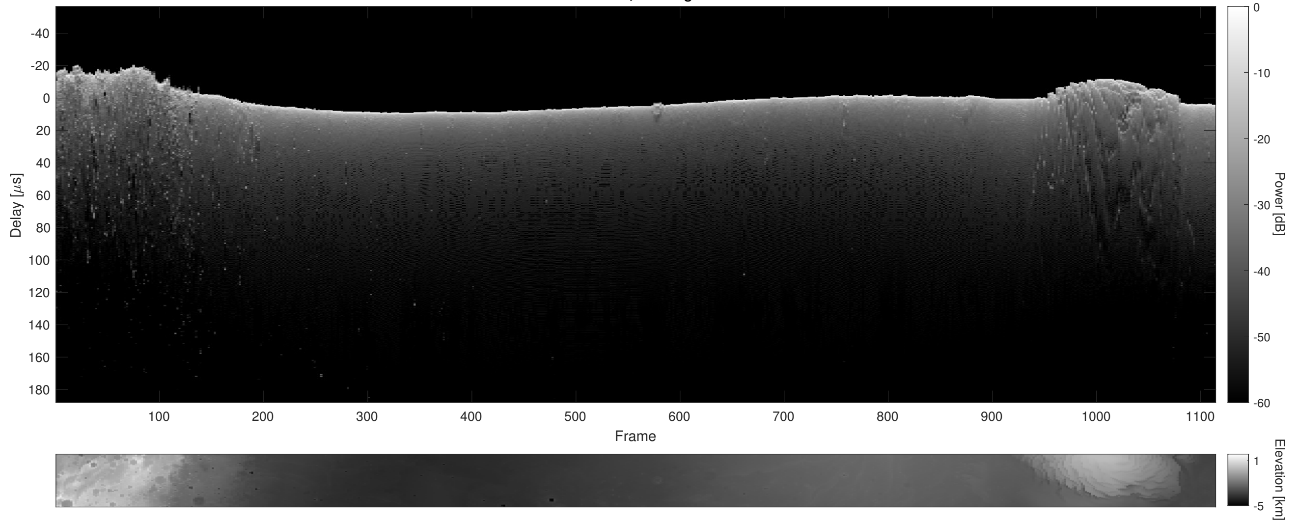
Orbit 14204, Cluttergram
