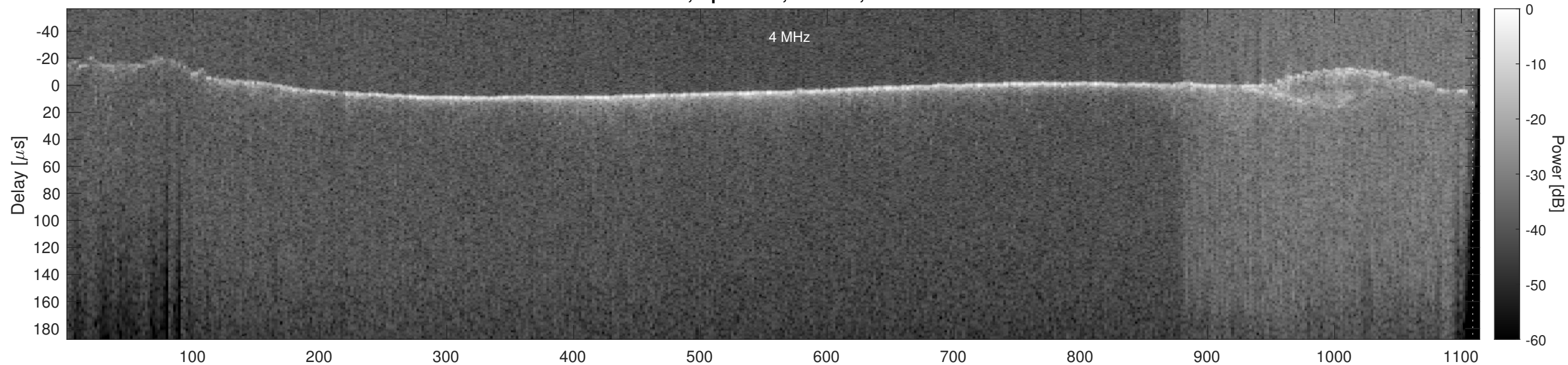
Orbit 14204, Optimized, Window, Channel 2
