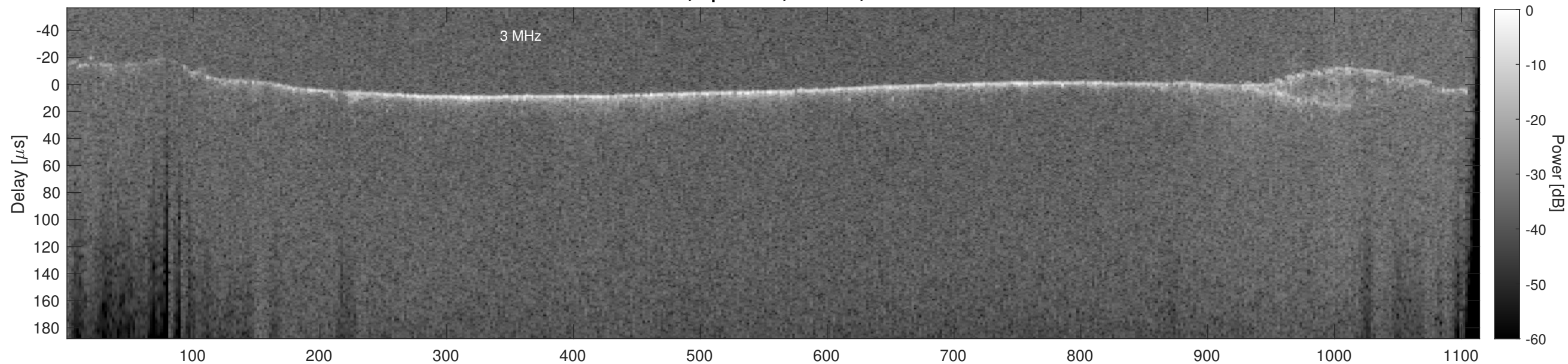
Orbit 14204, Cluttergram
