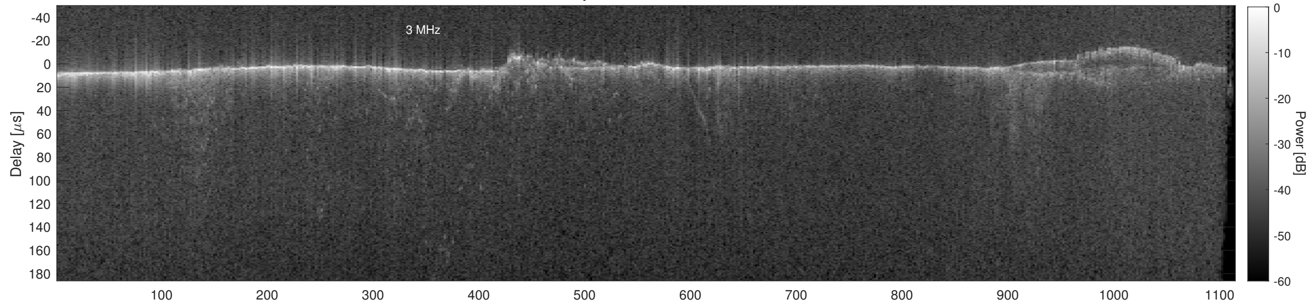
Orbit 14207, Cluttergram
