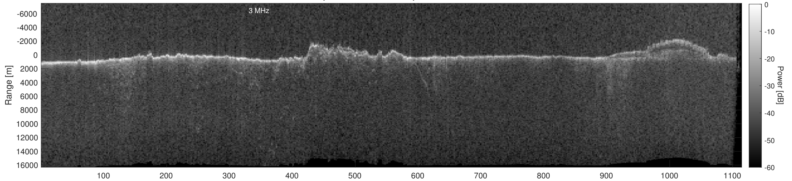
Orbit 14207, Depth-Corrected Cluttergram
