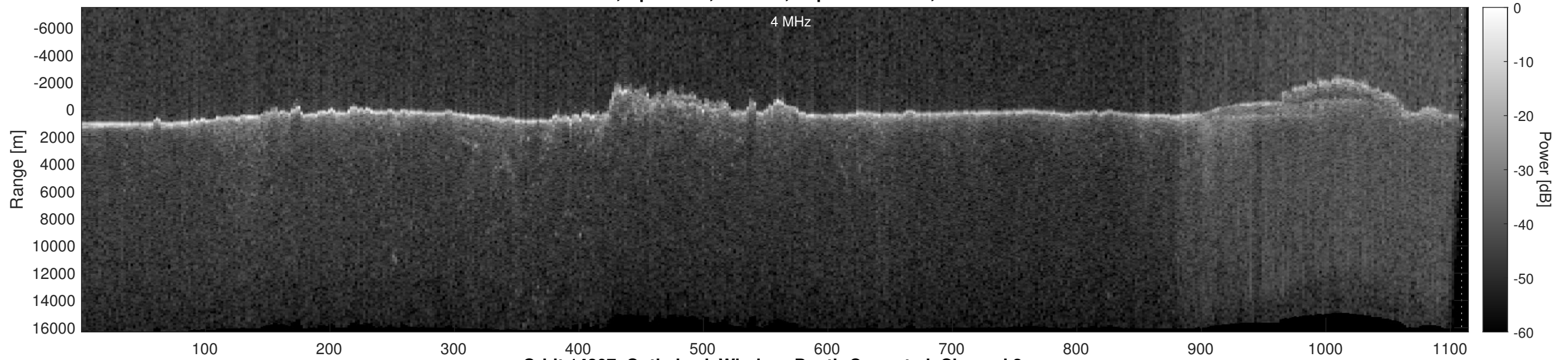
Orbit 14207, Optimized, Window, Depth-Corrected, Channel 2
