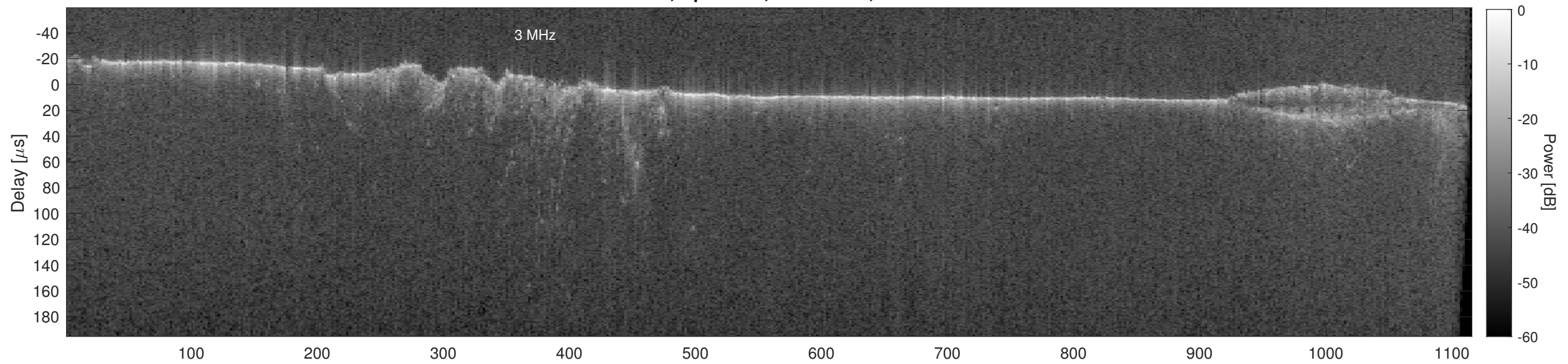
Orbit 14208, Cluttergram
