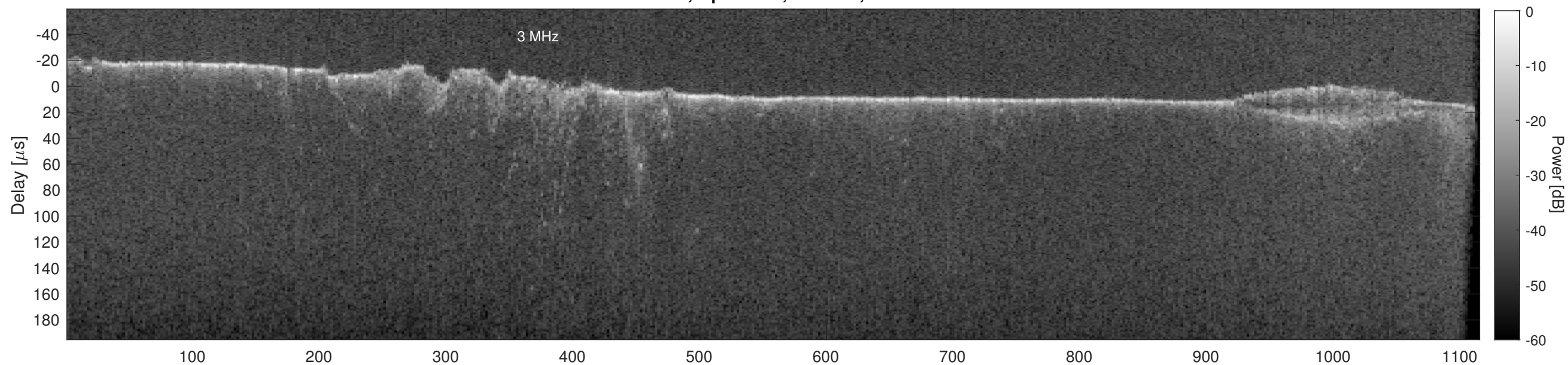
Orbit 14208, Cluttergram
