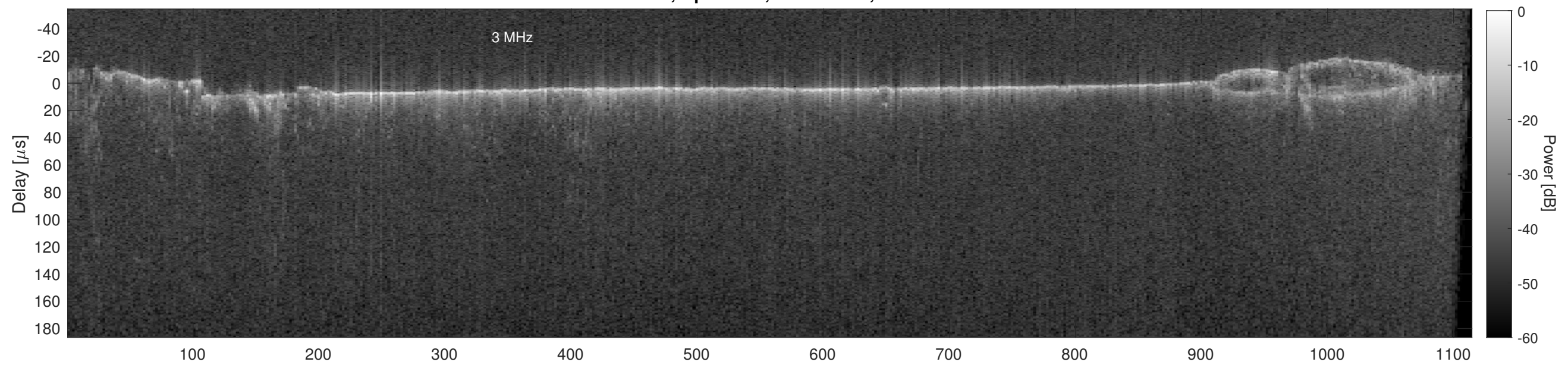
Orbit 14209, Cluttergram
