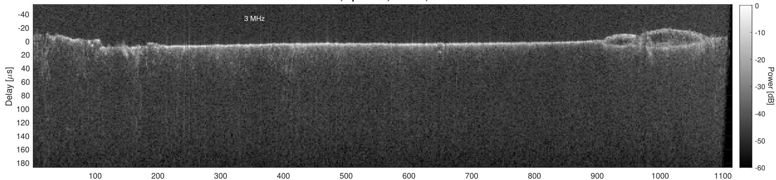
Orbit 14209, Cluttergram
