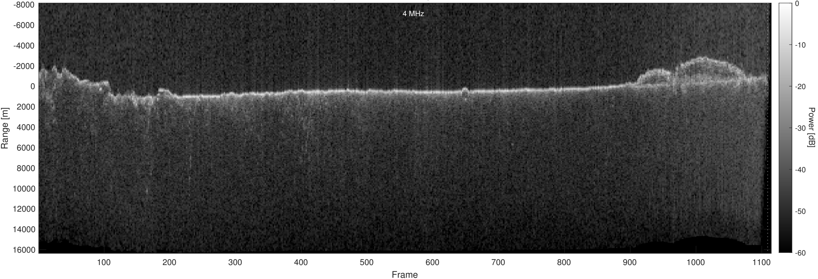
Orbit 14209, Optimized, Window, Depth-Corrected, Channel 2
