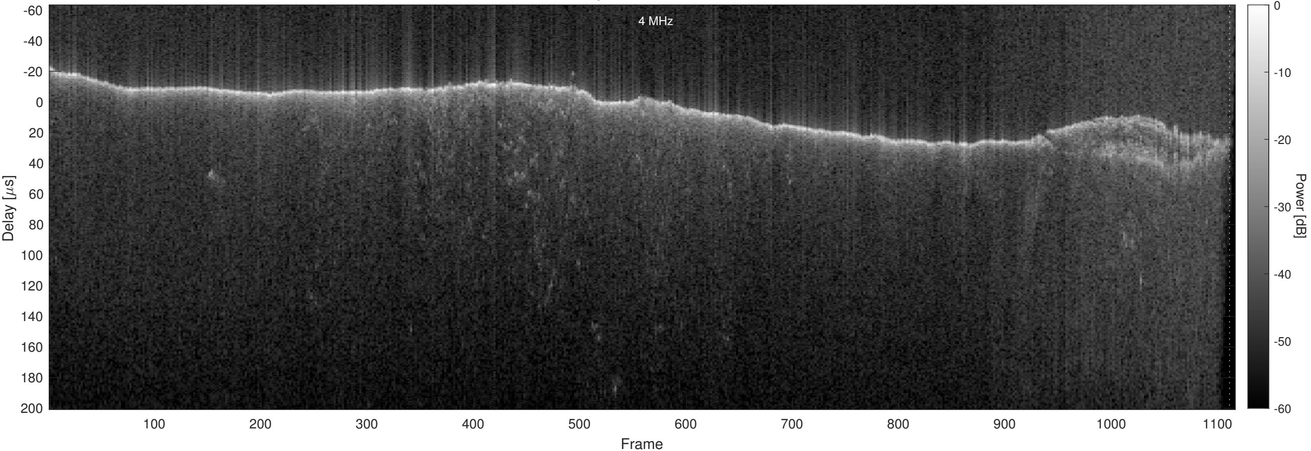
Orbit 14213, Chapman, No Window, Channel 2
