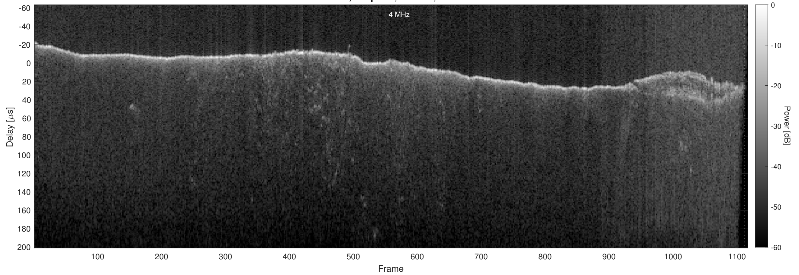
Orbit 14213, Chapman, Window, Channel 2
