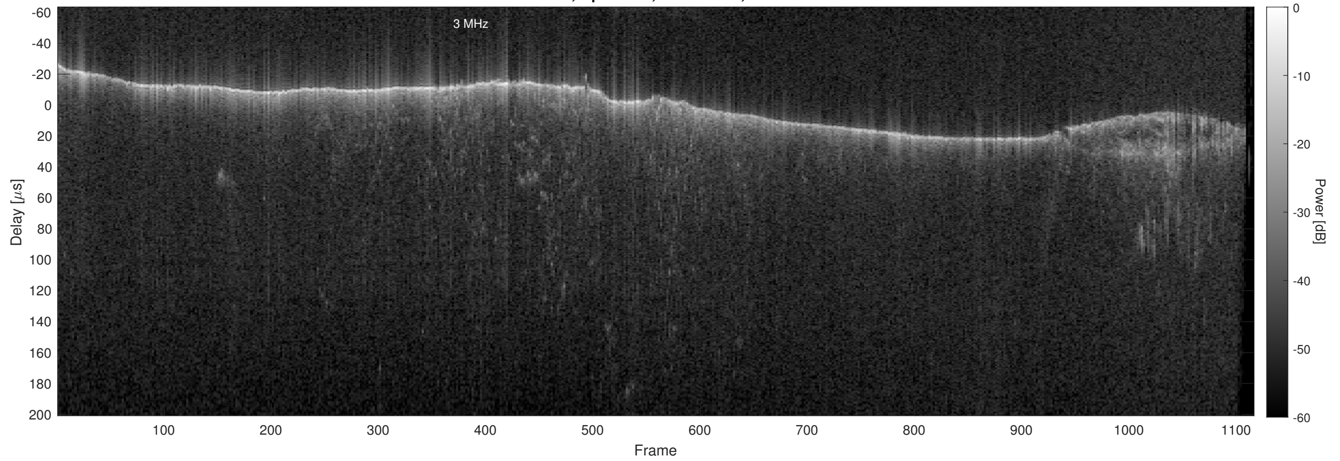
Orbit 14213, Optimized, No Window, Channel 2
