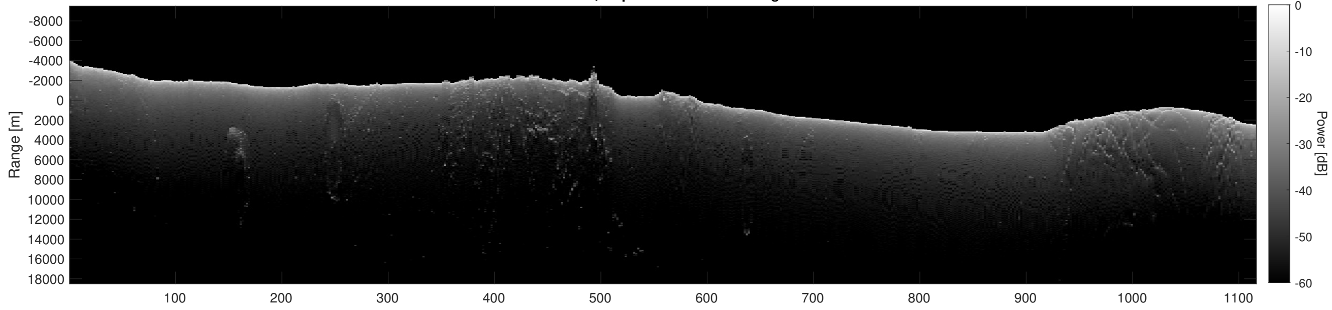
Orbit 14213, Depth-Corrected Cluttergram
