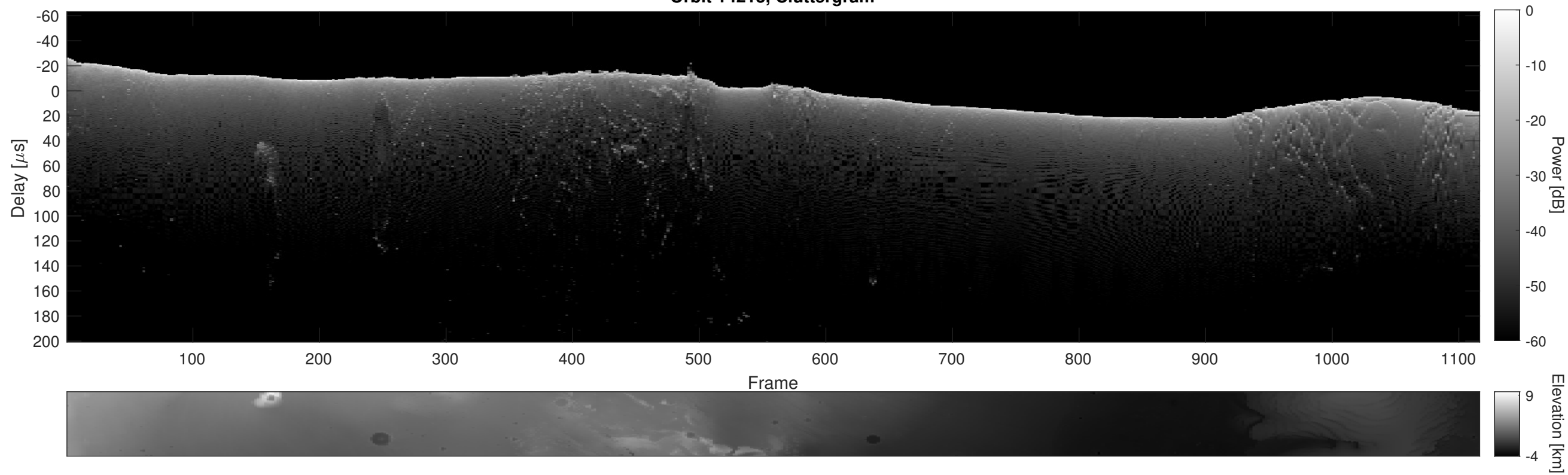
Orbit 14213, Cluttergram
