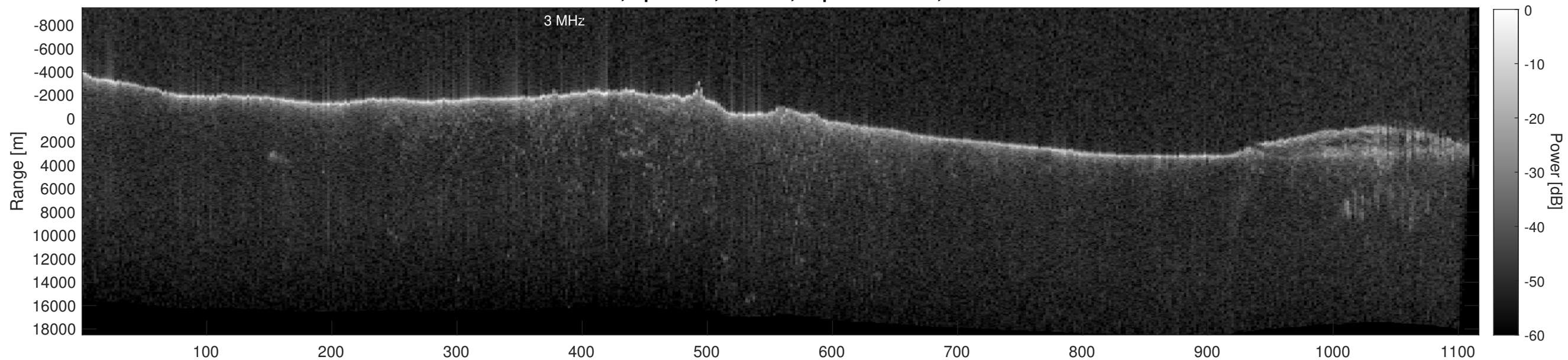
Orbit 14213, Depth-Corrected Cluttergram
