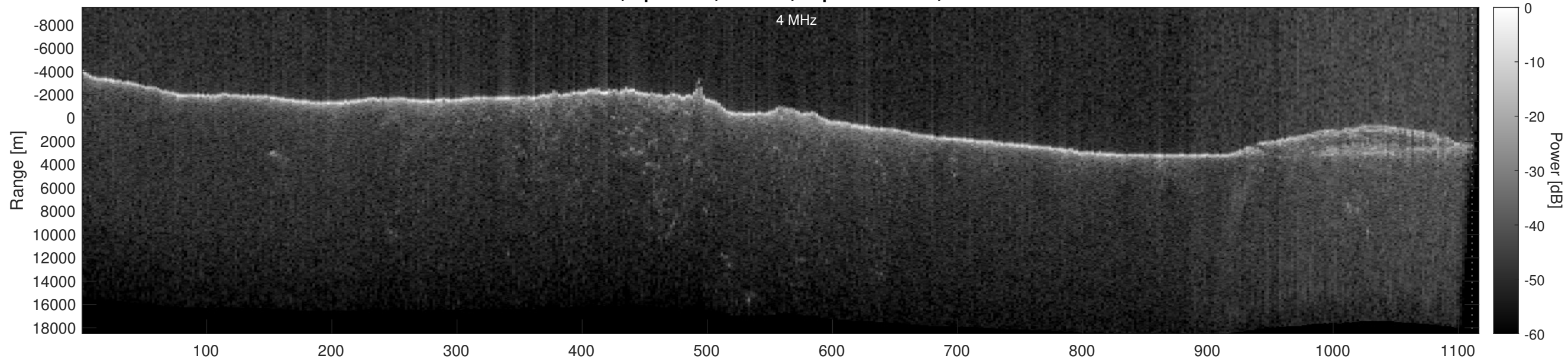
Orbit 14213, Optimized, Window, Depth-Corrected, Channel 2
