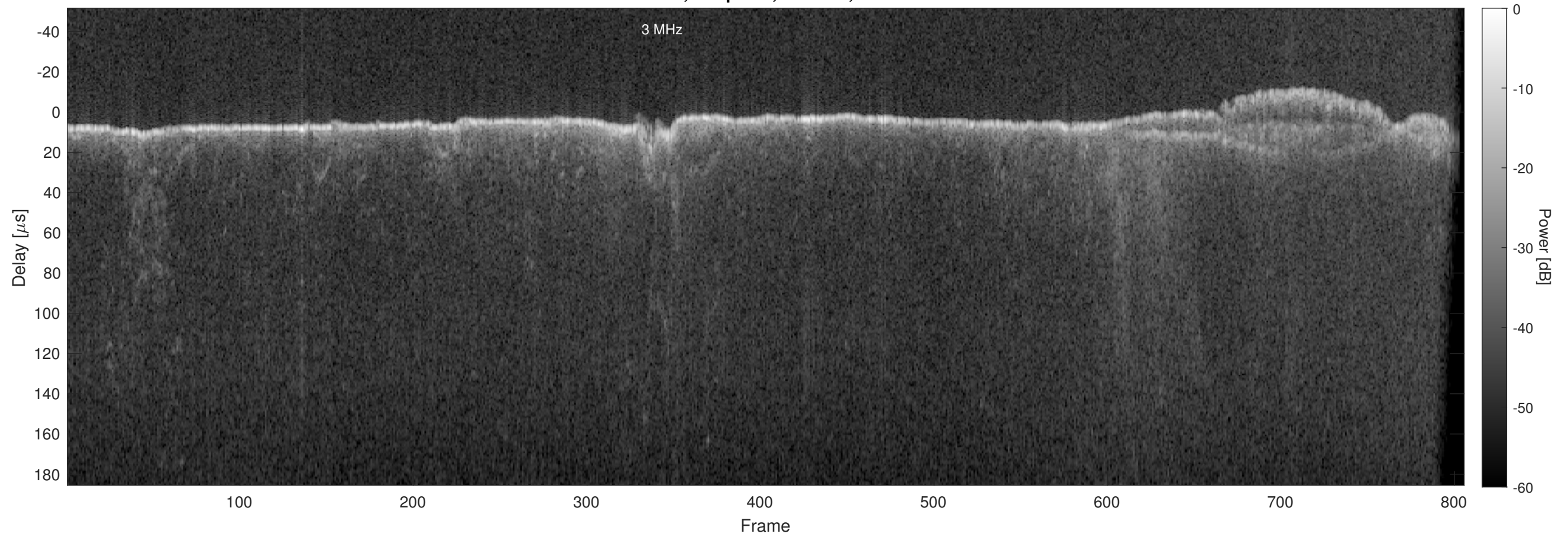
Orbit 14214, Chapman, Window, Channel 2
