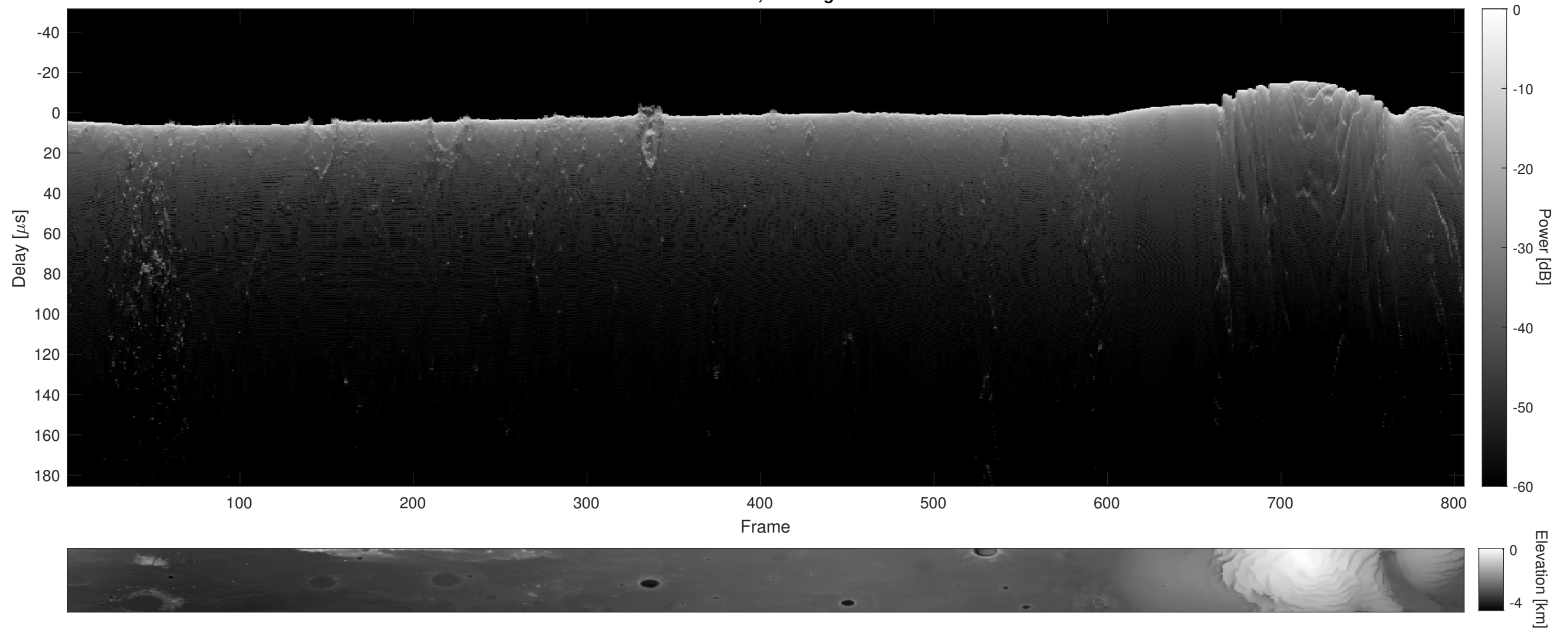
Orbit 14214, Cluttergram
