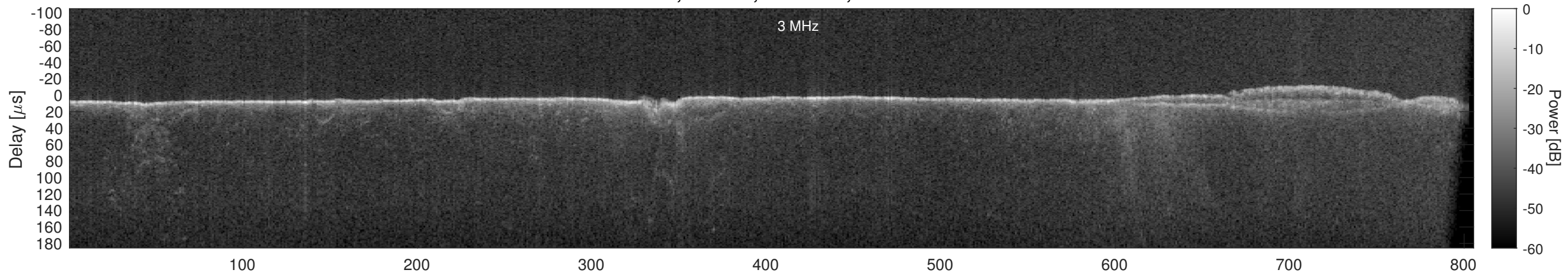
Orbit 14214, Window, Channel 2, Chapman
