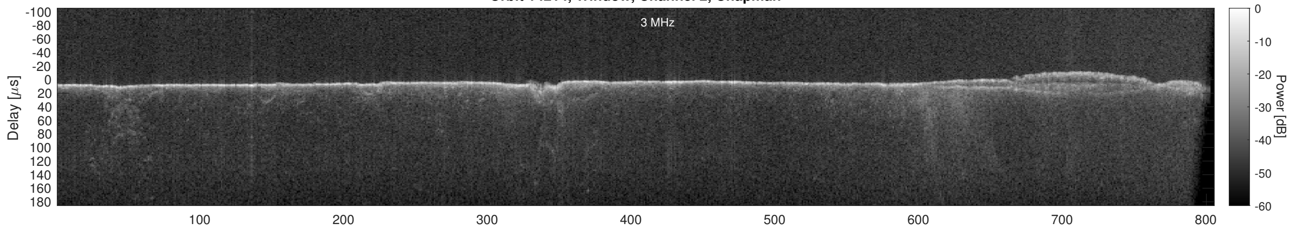
Orbit 14214, Window, Channel 2, Optimized
