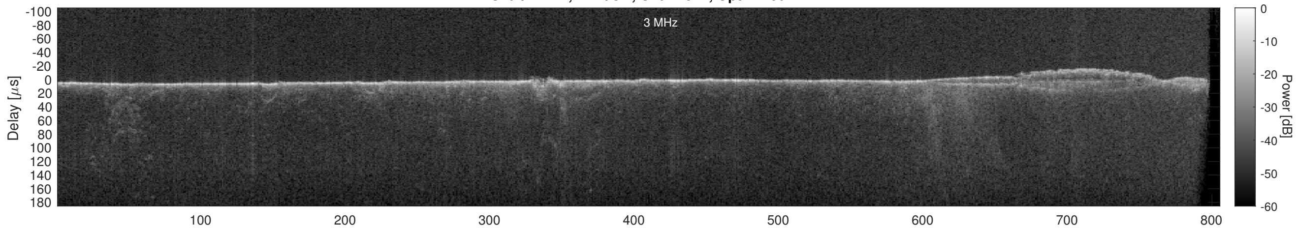
Orbit 14214, Cluttergram
