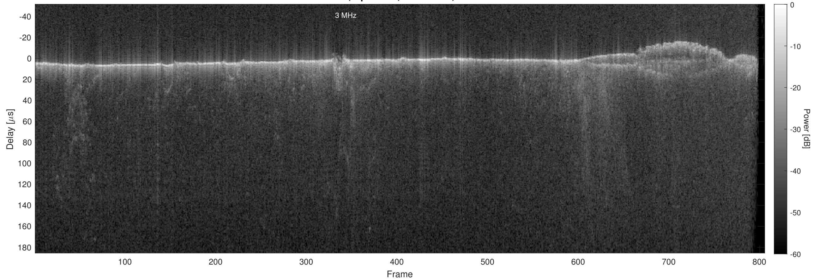
Orbit 14214, Optimized, No Window, Channel 2
