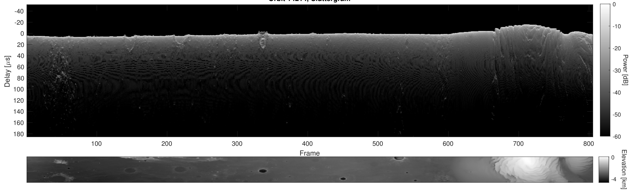
Orbit 14214, Cluttergram
