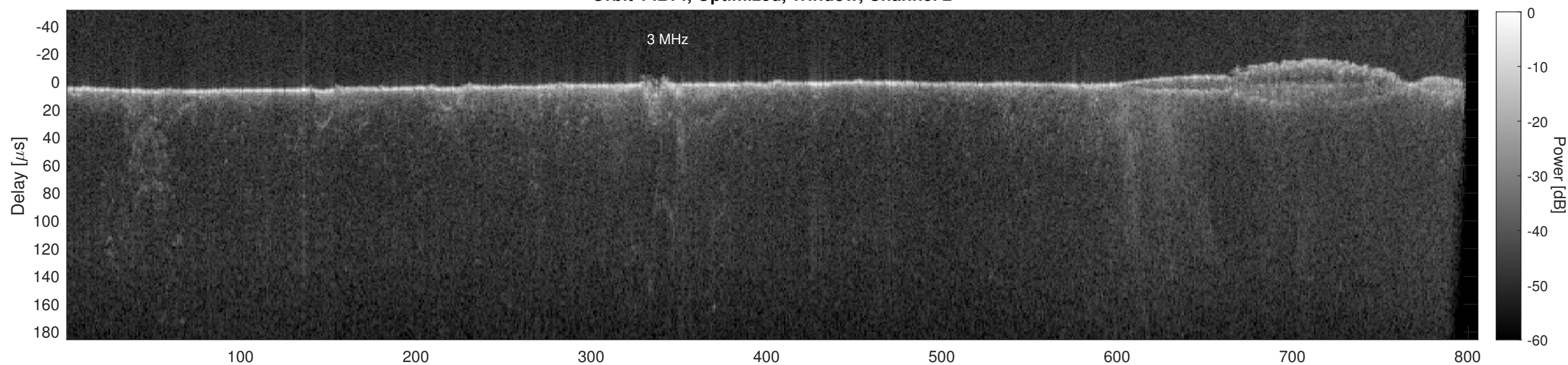
Orbit 14214, Cluttergram
