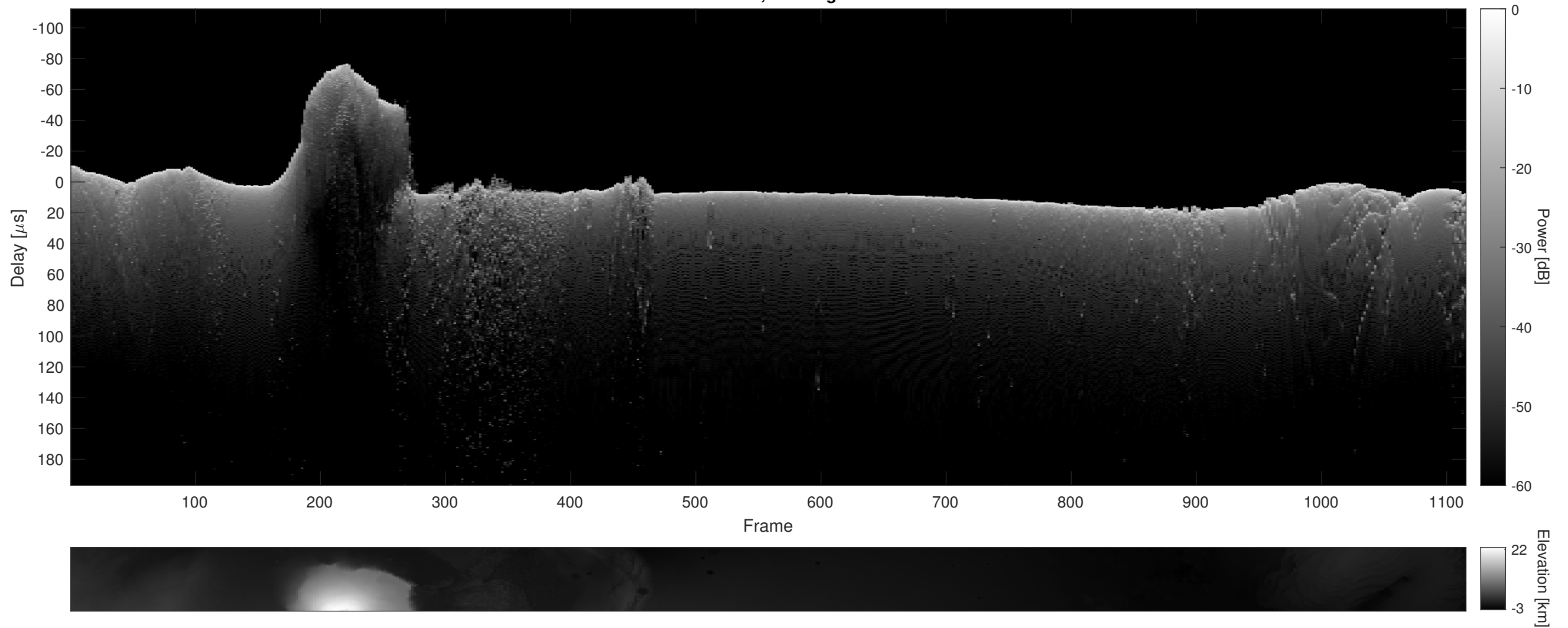
Orbit 14217, Cluttergram
