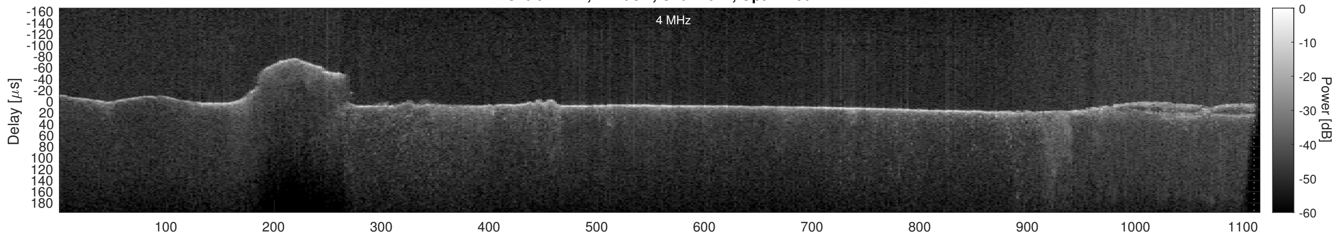
Orbit 14217, Cluttergram
