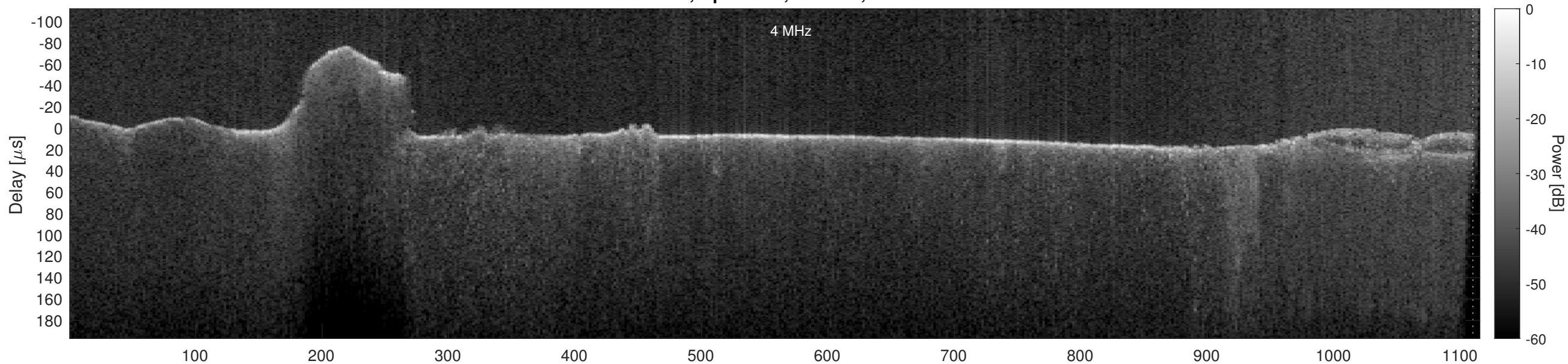
Orbit 14217, Optimized, Window, Channel 2
