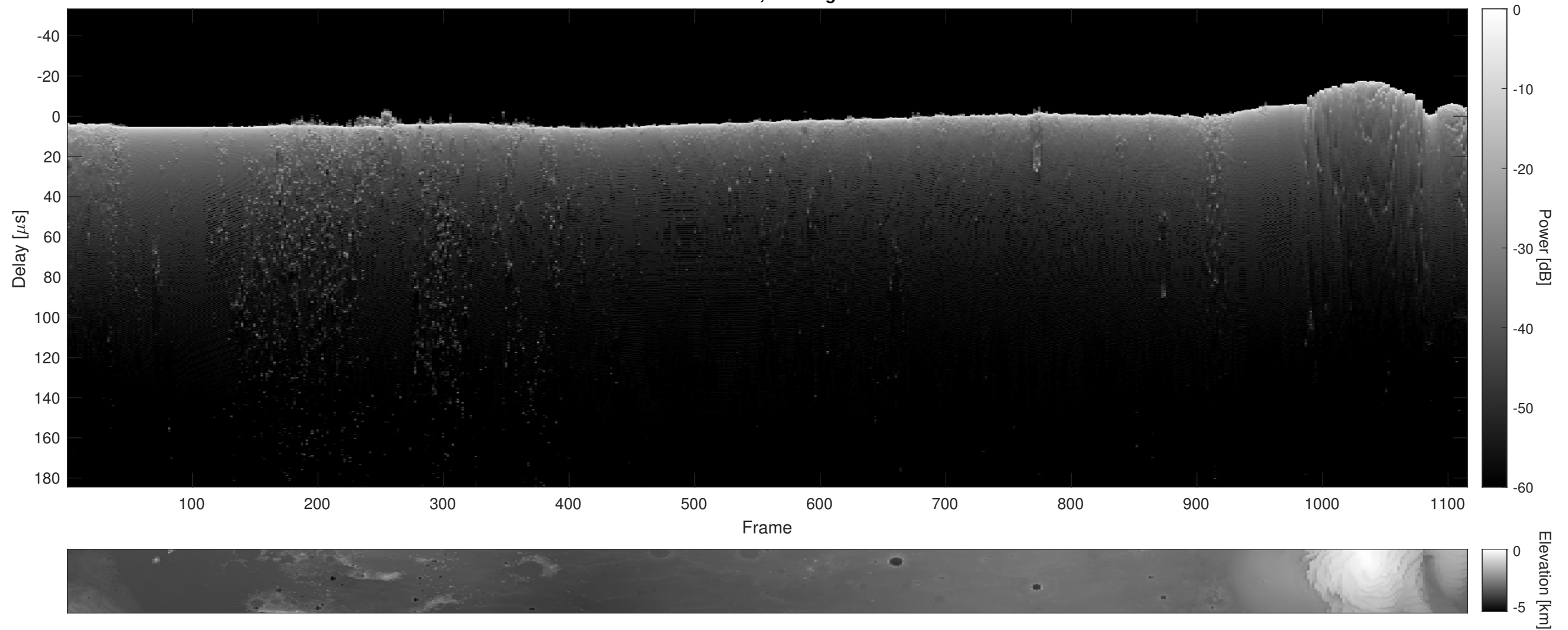
Orbit 14221, Cluttergram
