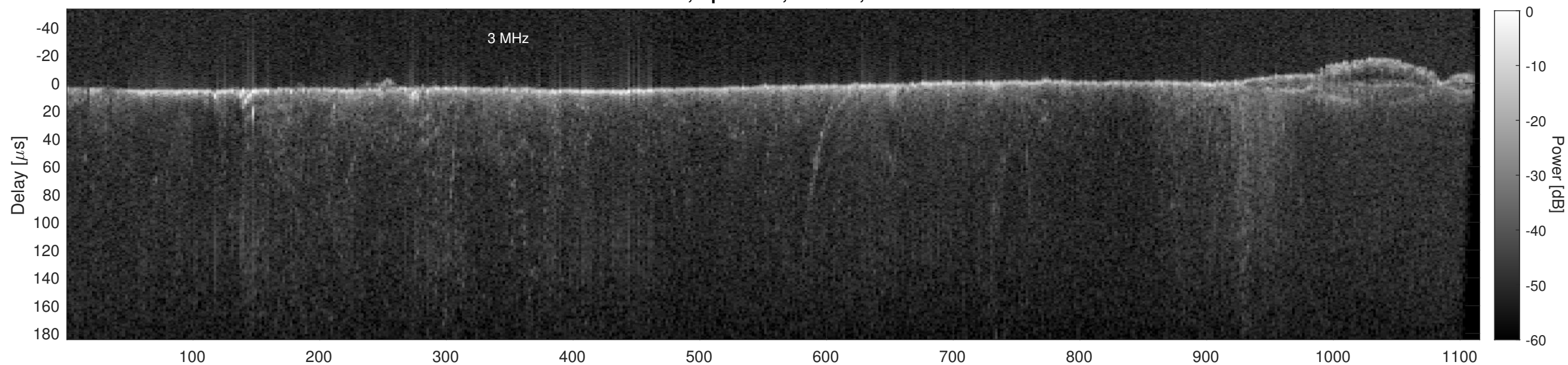
Orbit 14221, Cluttergram
