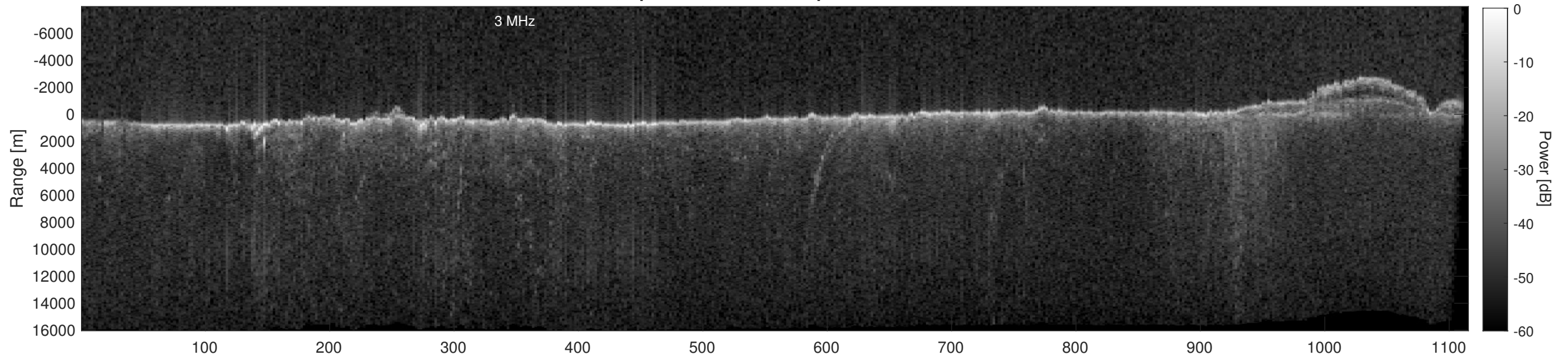
Orbit 14221, Depth-Corrected Cluttergram
