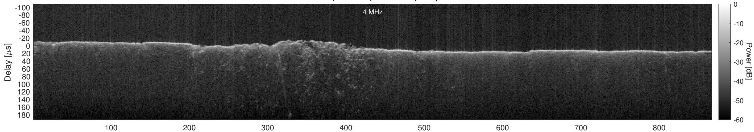
Orbit 14222, Window, Channel 1, Optimized
