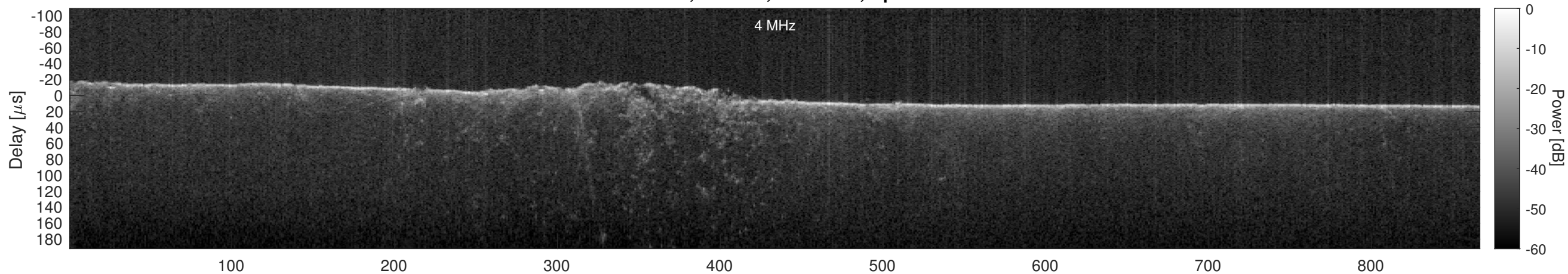
Orbit 14222, Cluttergram
