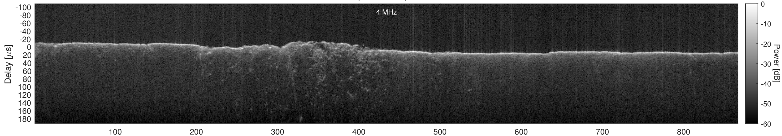
Orbit 14222, Window, Channel 1, Chapman
